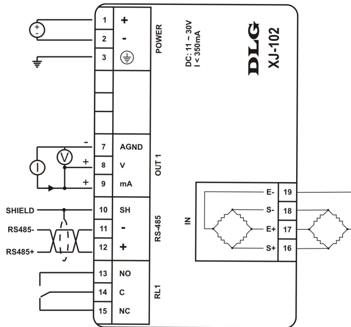
Figura 5 – Borneiras XJ-102/DC
